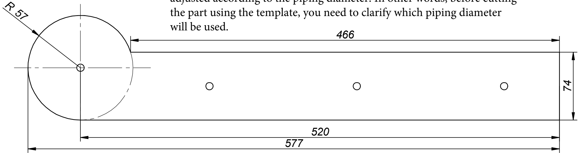
Template №9 10 mm plywood - 2
