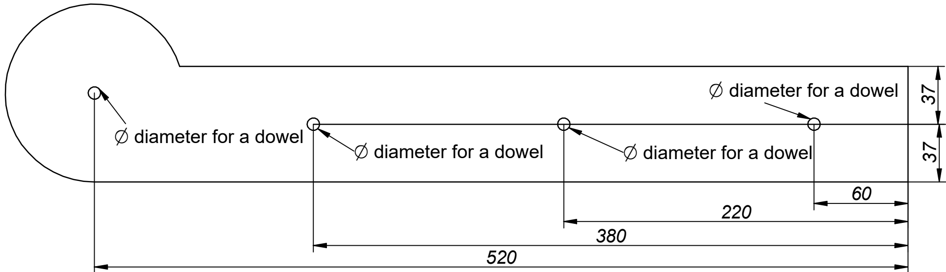
Template №9 10 mm plywood - 2
